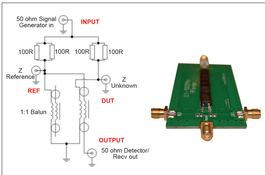
Fig. 8 - Return Loss Bridge
